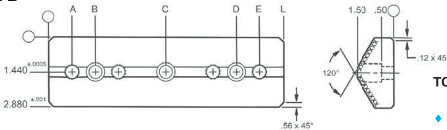
FIGURE C Assembly
